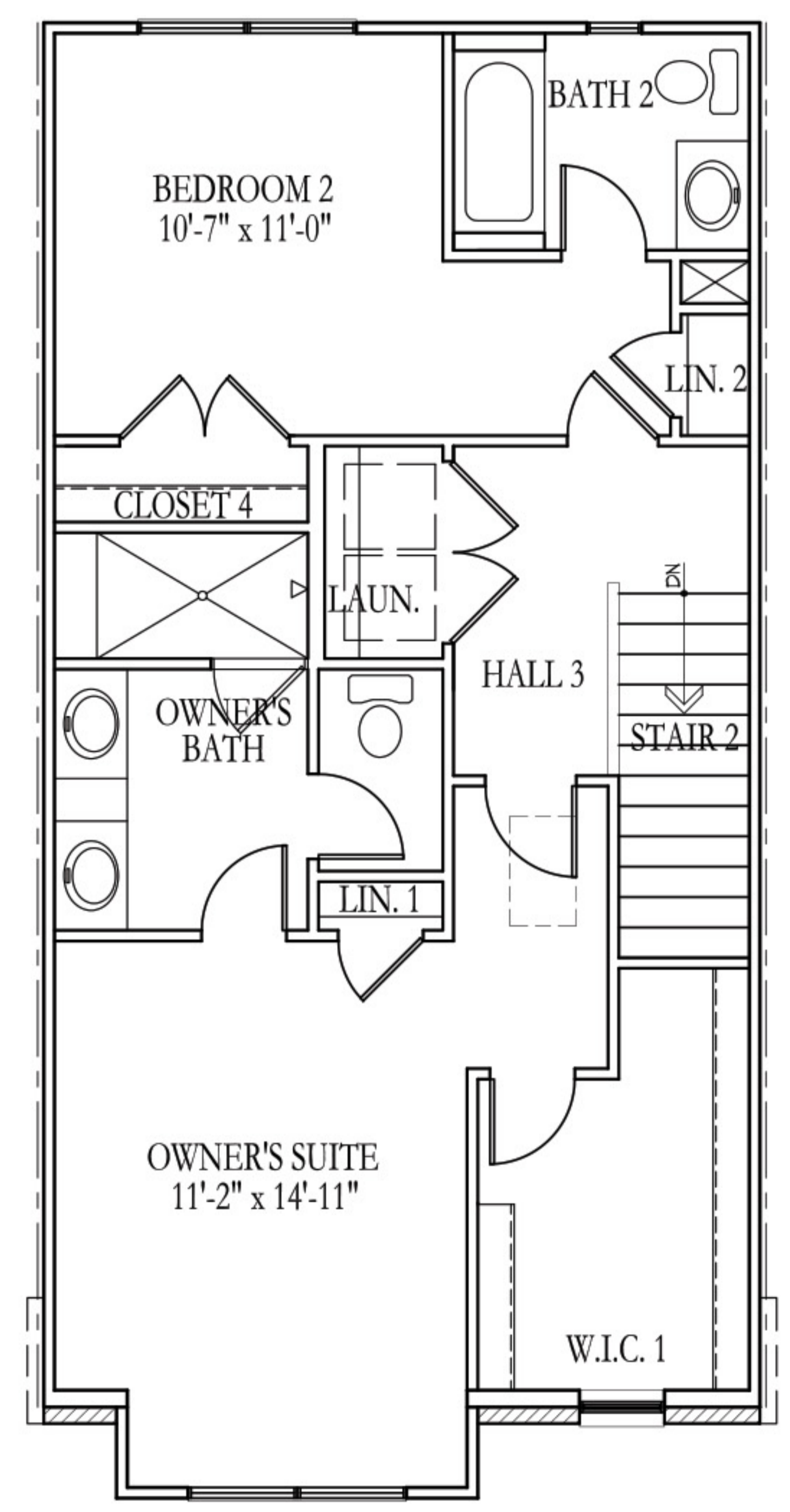
ALTERNATE THIRD FLOOR PLAN
