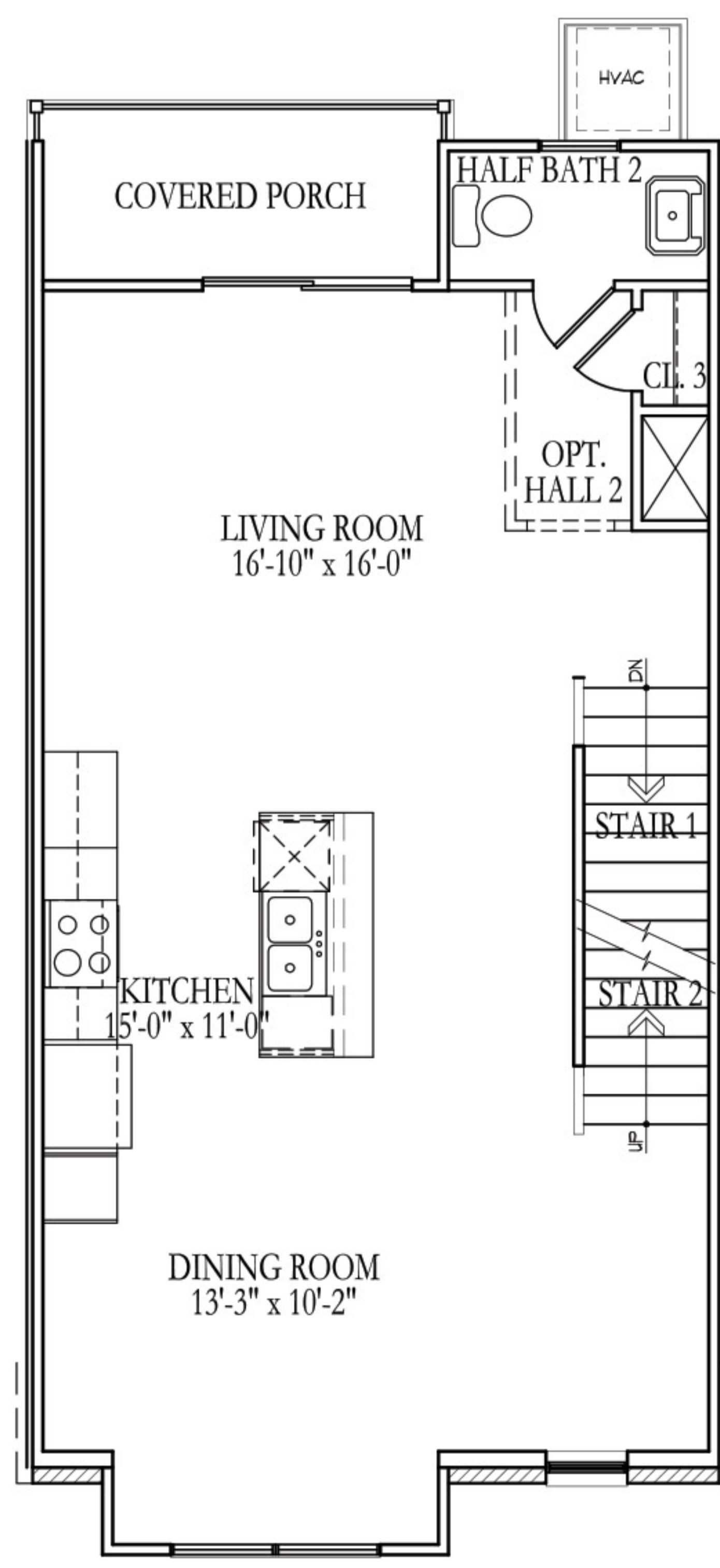
ALTERNATE SECOND FLOOR PLAN
