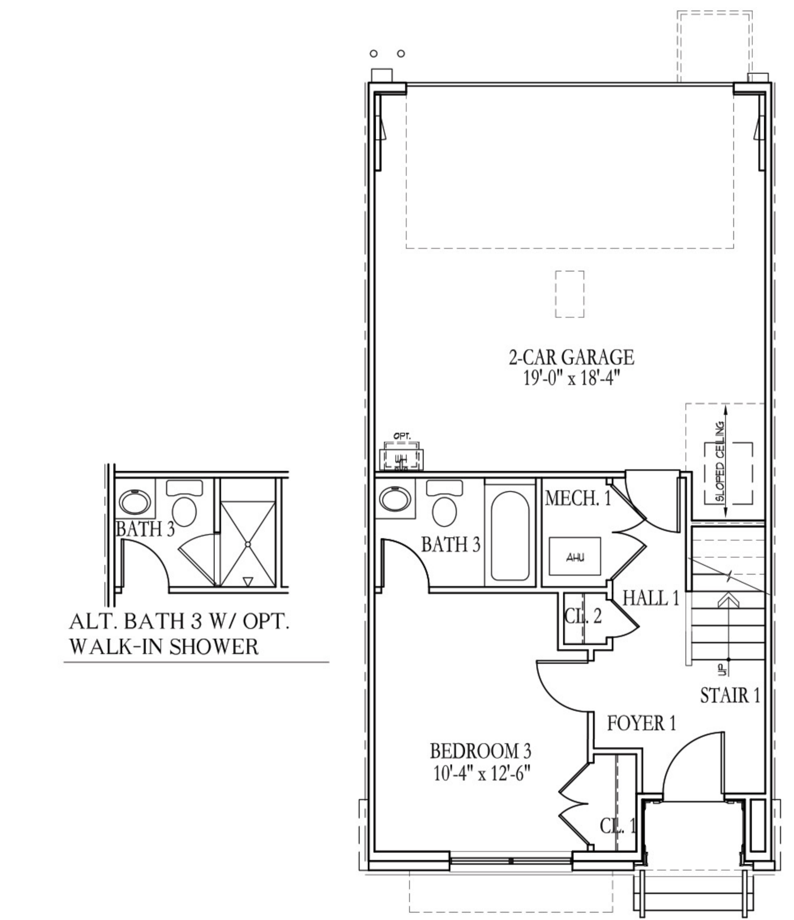
ALTERNATE FIRST FLOOR PLAN
